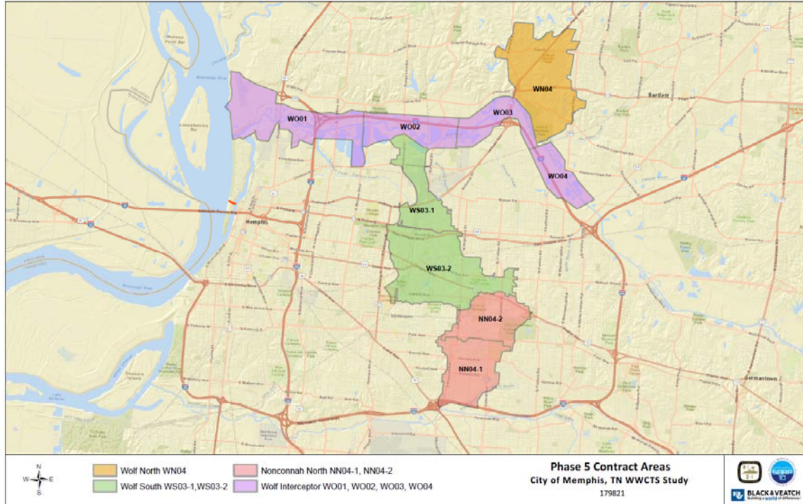
Figure 1: Sewer Assessment & Rehabilitation Program Phase 5 Areas
